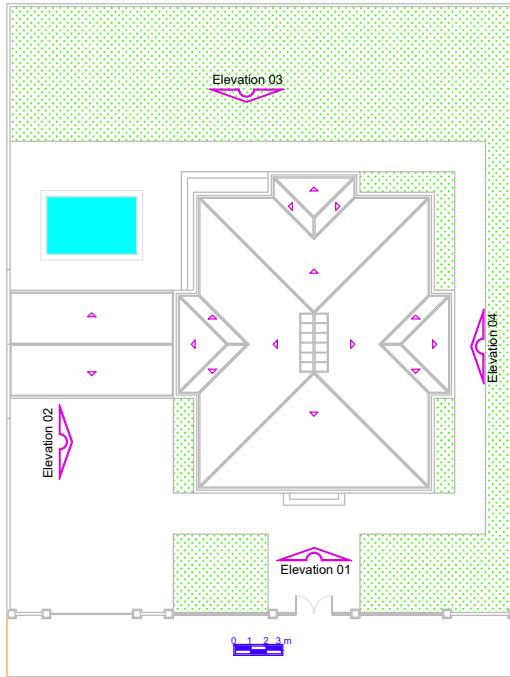
Roof Plan
